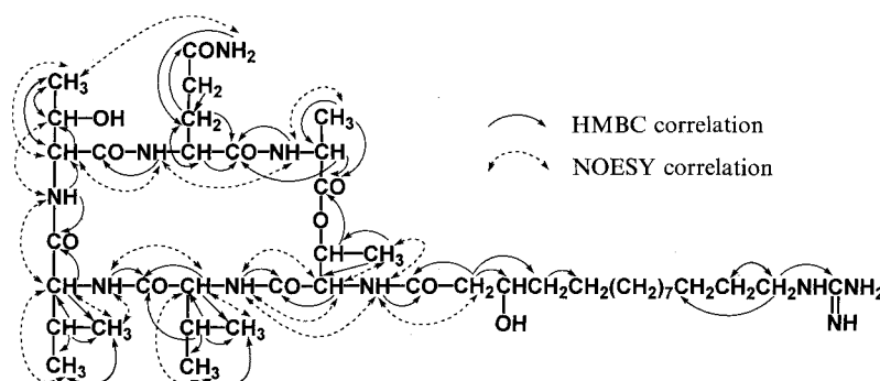
Fig. 7. HMBC and NOESY correlations for fusaricidin B (1).
