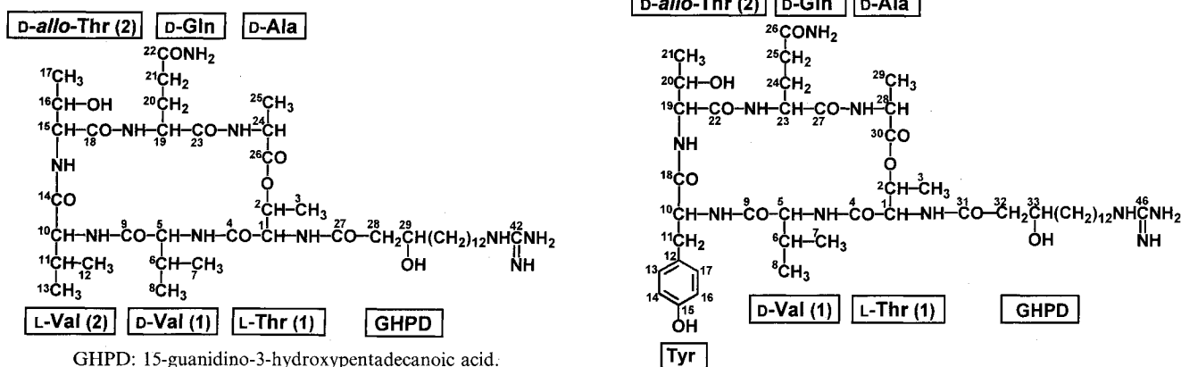
Fig. 3. Structure of fusaricidin D (3).
